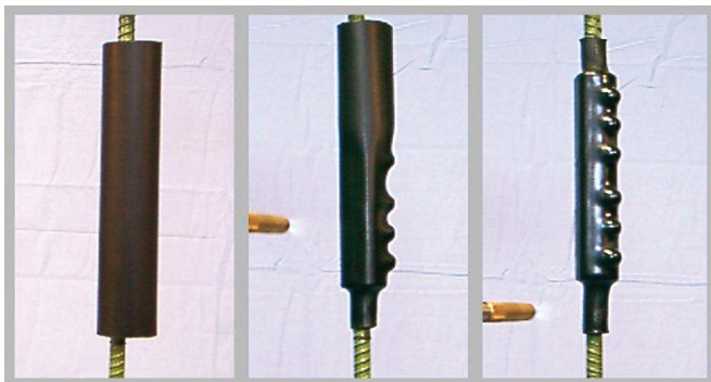
SpliceSeal is applied in seconds, using a hand-held torch. Bar Lock couplers shown.
